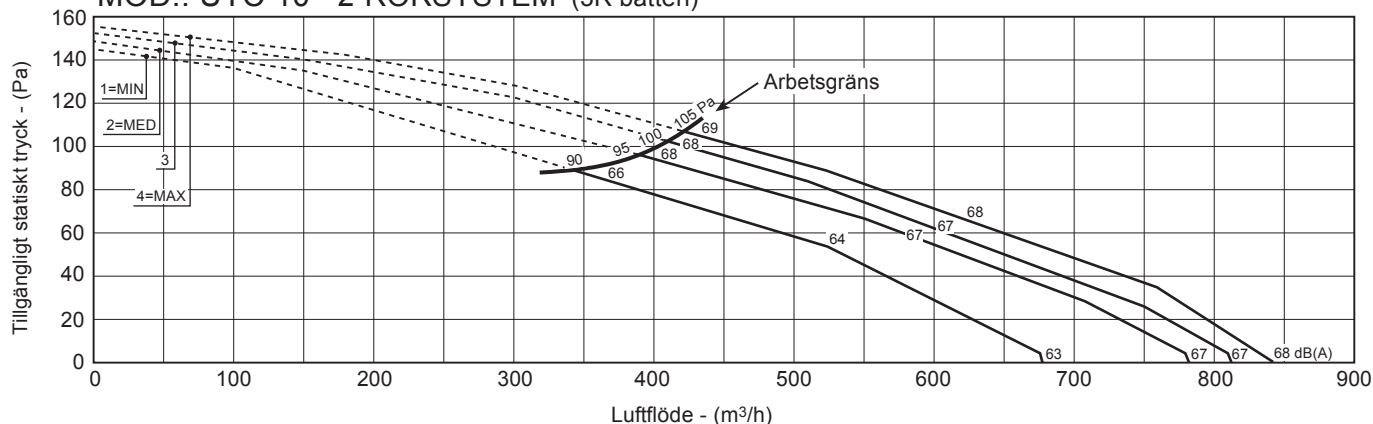
MOD.: UTC 20 - 2-RÖRSYSTEM (3R batteri)
