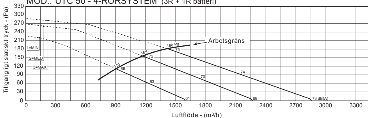
MOD.: UTC 60 - 4-RÖRSYSTEM (4R + 2R batteri)
