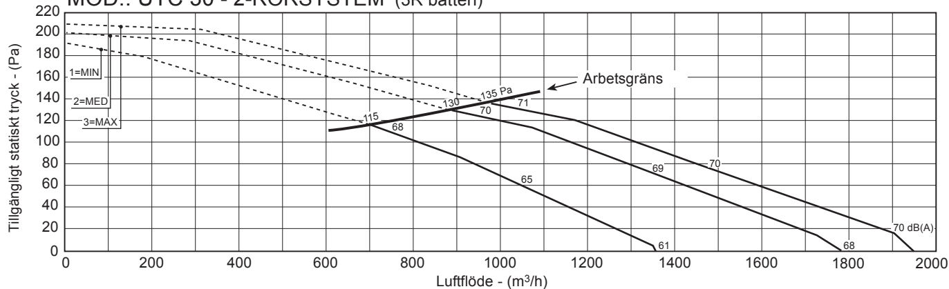
MOD.: UTC 30 - 2-RÖRSYSTEM (3R batteri)
